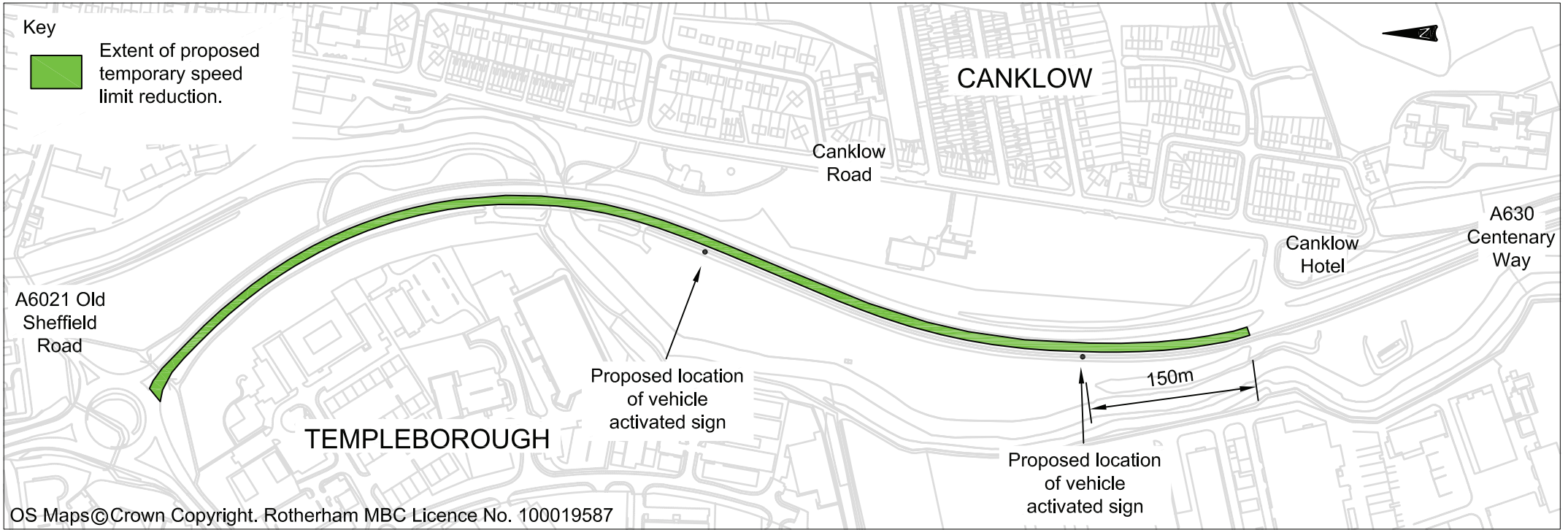
Extent of proposed temporary 40mph speed limit Not to scale
